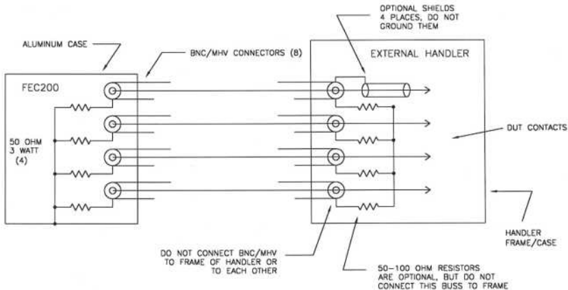
IDEAL CONNECTION OF HANDLER TO FEC200 TESTER FOR BEST NOISE IMMUNITY AND ACCURACY
